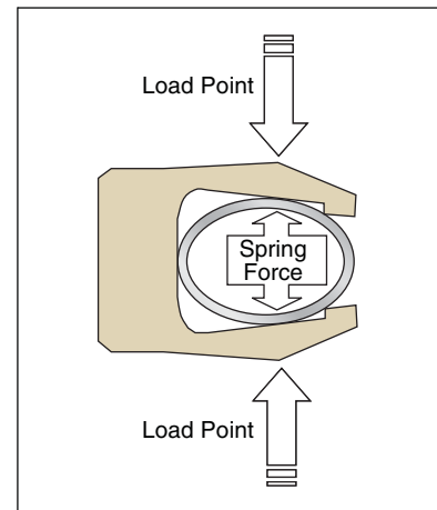
Figure 2-16. Installed State
