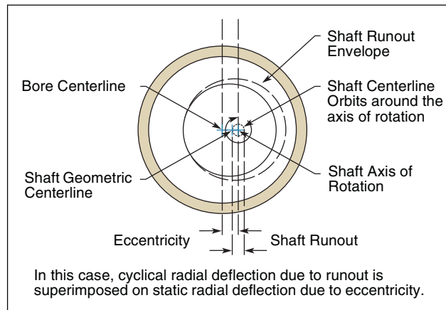
Figure 2-12. Shaft Runout
