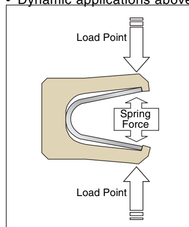
Figure 2-15. Installed State
