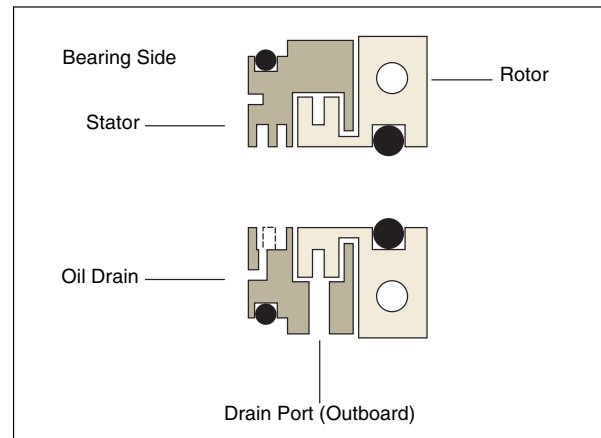
Figure 8-2. Position the Rotor Halves
