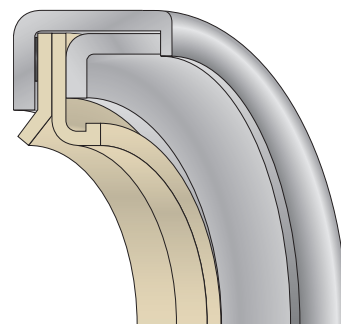
FlexiCase Rotary Seal
