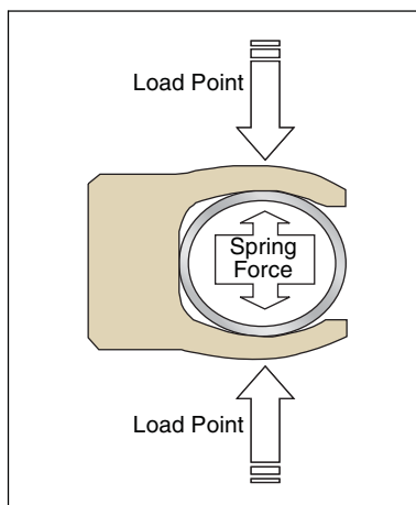
Figure 2-17. Installed State
