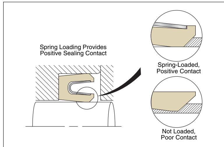
Figure 2-13. Spring Loading
