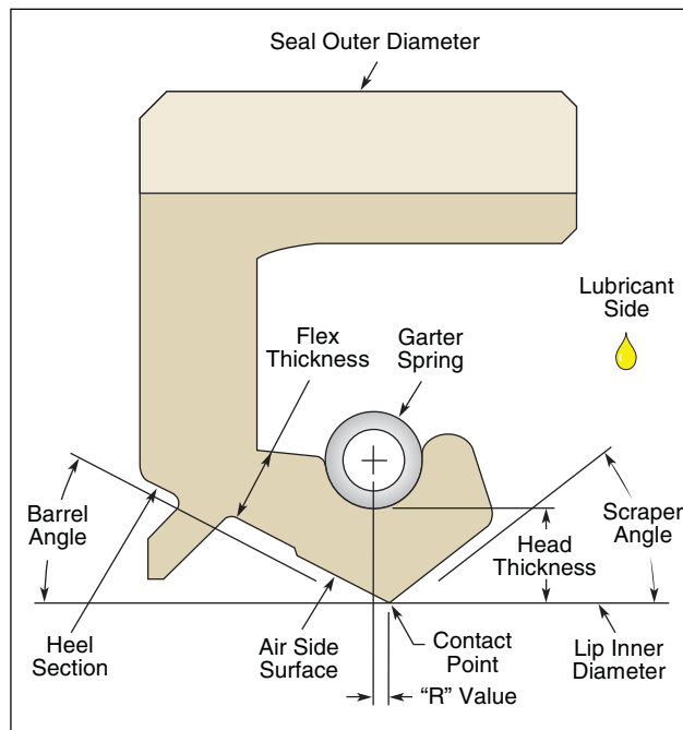
Figure 2-2. Seal Components
