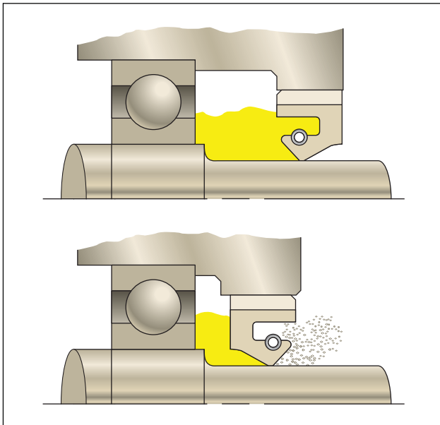
Figure 2-3. Installations Facing Lubricant and Contaminant
