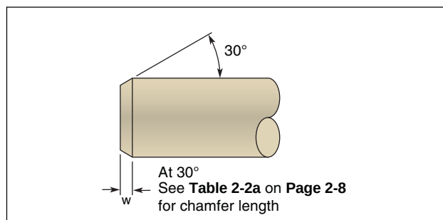
Figure 2-18. Shaft Profile
