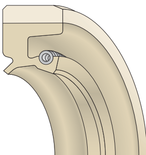
Clipper Oil Seal
