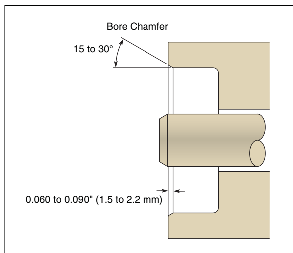
Figure 6-2. Housing Profile
