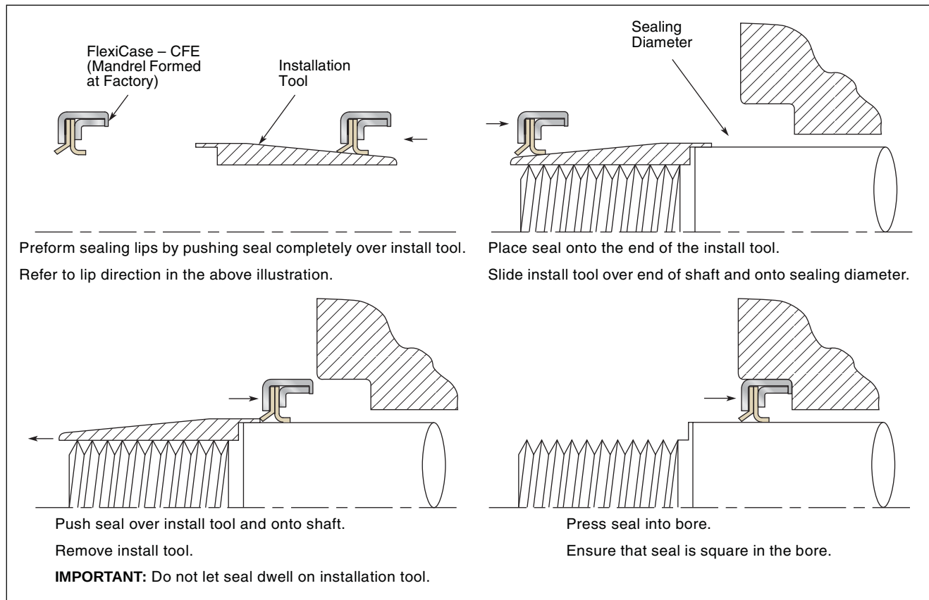
Figure 10-1. FlexiCase Installation
