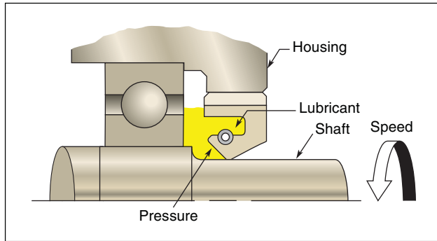
Figure 2-5. Sealing System
