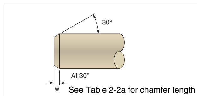
Figure 2-7. Shaft Profile
