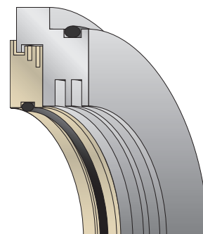
ProTech Bearing Isolator
