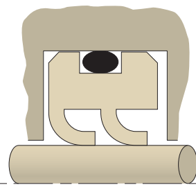
FlexiLip in air conditioning compressor 260 sfpm, 20 - 300 psi
