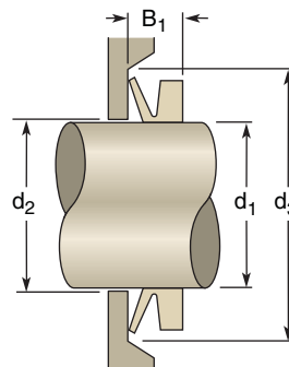
Assembly Dimensions
