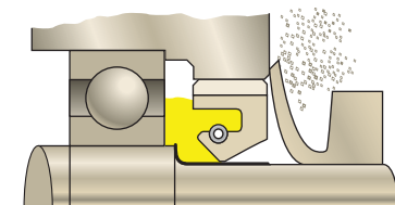
V-Seal with Primary Seal and Quick Sleeve
