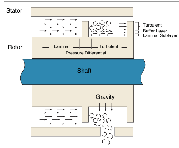
Figure 8-1. Effects of Turbulence
