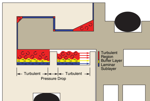
Pressure Drops and Turbulence
