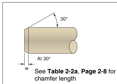
Figure 5-1. Shaft Profile
