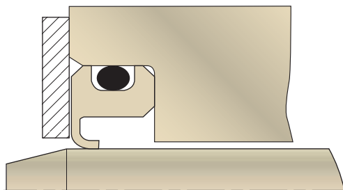
FlexiLip with Retainer for Higher Pressure
