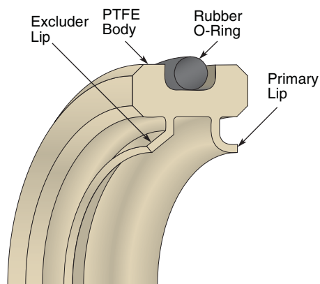
FlexiLip Components
