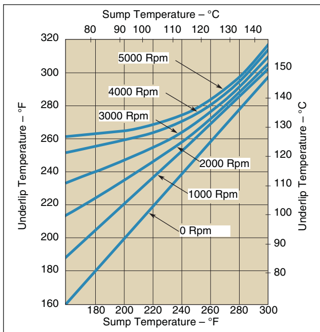
Figure 2-8. Example Shaft Conditions
