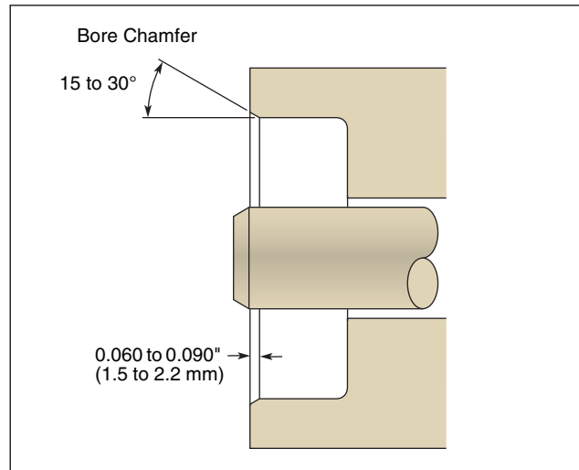
Figure 2-10. Housing Profile
