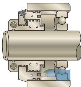
Split Air Purge
