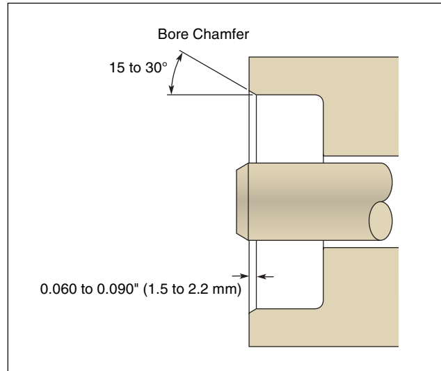
Figure 2-19. Housing Profile
