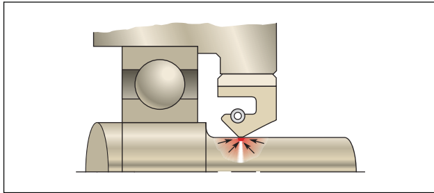
Figure 2-9. Internal Pressure
