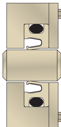
FCC-V in Two-Piece Gland
