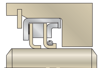
FlexiCase in Gland
