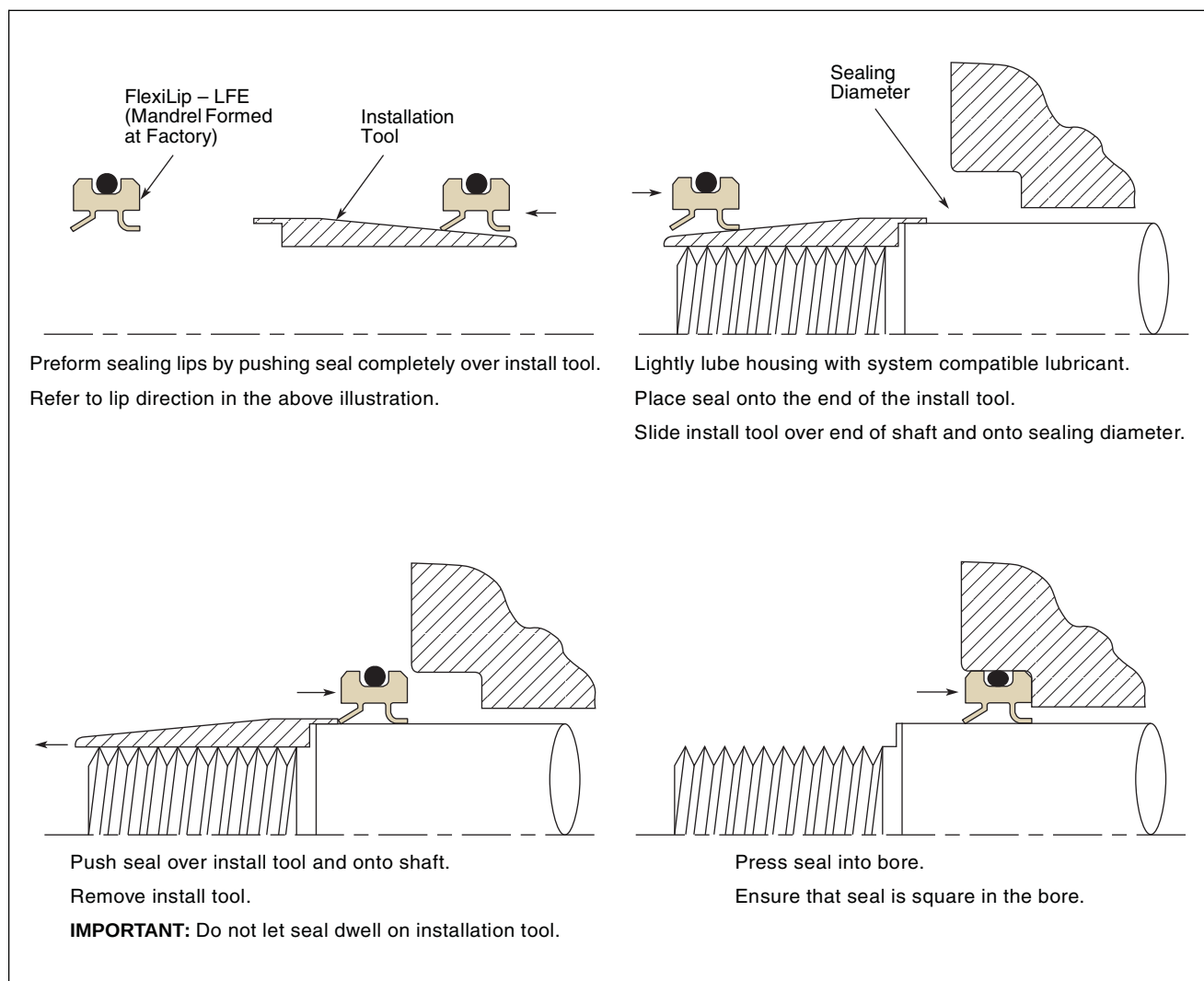
Figure 9-1. FlexiLip Installation
