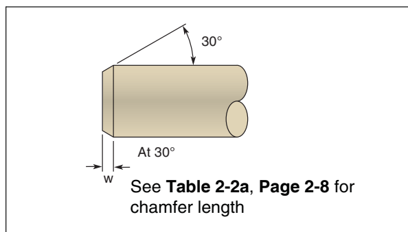
Figure 6-1. Shaft Profile
