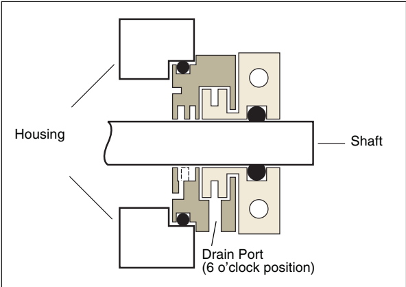
Figure 8-3. Proper Installation
