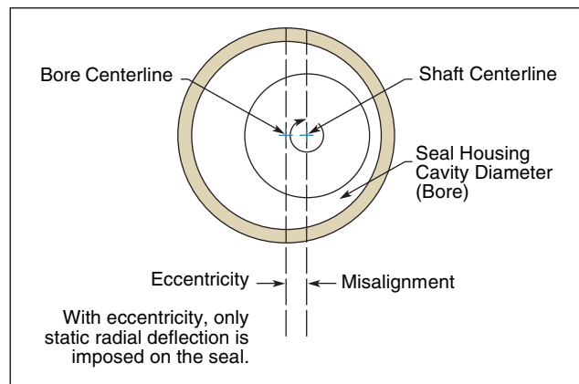
Figure 2-11. STBM
