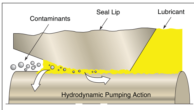
Figure 2-1. Rotary Shaft Seal at Work
